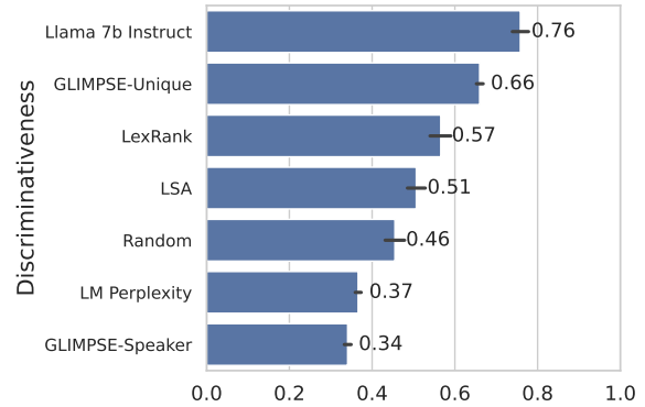
(a) Discriminativeness.
