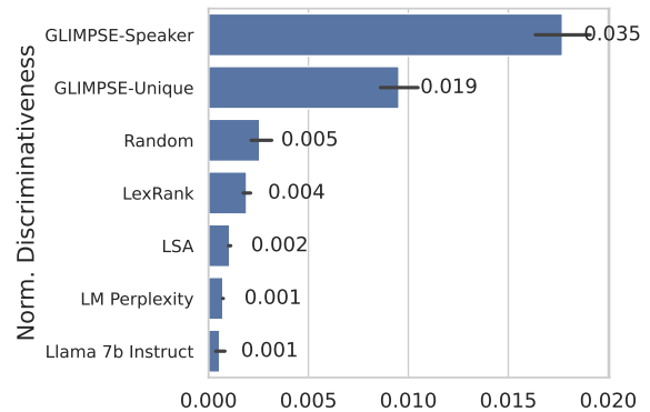
(b) Discriminativeness per character.
