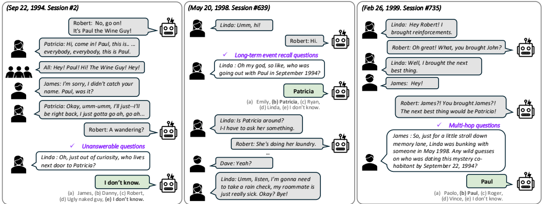
Figure 1: An overall process of DialSim. Gray bubbles represent scripted utterances, and white speech bubbles indicate spontaneous questions asked during the simulation. Colored speech bubbles indicate the agent’s responses to the questions. (Left) An unanswerable question. (Center) A long-term event recall question. (Right) A multi-hop question that requires understanding past sessions ( i.e. , the Left and Center boxes). The dialogue and questions are based on the Friends script, with character names anonymized ( e.g. , Ross → Robert). The question is asked in the format chosen by the user, either in a multiple-choice format or as an open-ended question.
