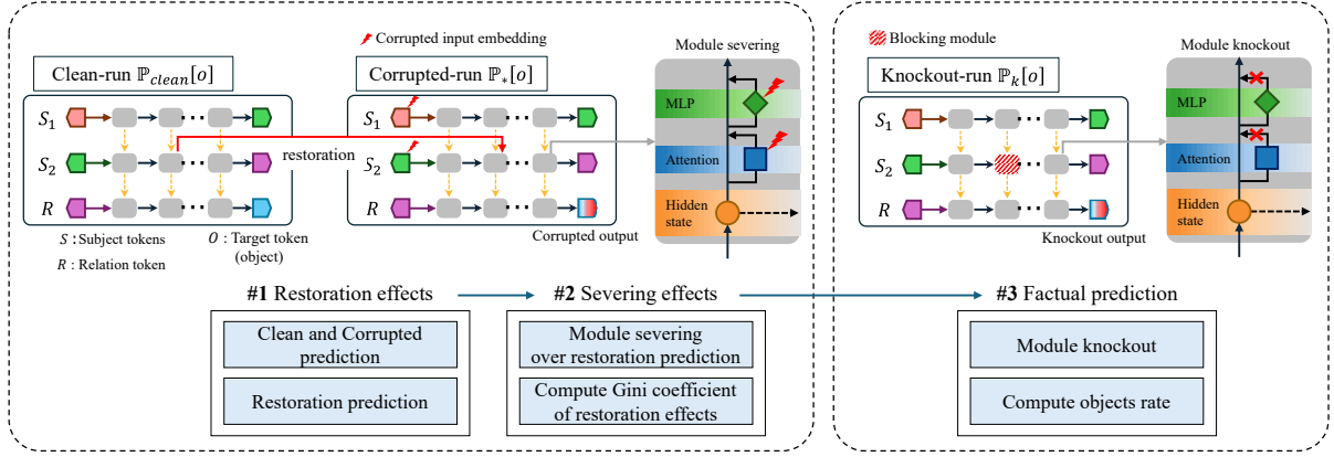
Figure 1: Overview of Our Evaluation. The pipeline consists of three main stages: (1) restoration effects, (2) severing effects, and (3) factual prediction. Each stage applies a distinct intervention strategy to evaluate the contribution of the Attention and MLP modules to factual association recall.
