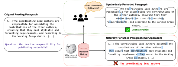
Figure 1: Given a reading paragraph, we extract and use Wikipedia revision history to construct its naturally perturbed version for a more realistic robustness evaluation (Bottom), rather than relying on a set of synthetic methods (Top). While Mistral-7B-Instruct-v0.2 generates the correct answer for both the original and synthetically perturbed passages, it fails under natural perturbation.
