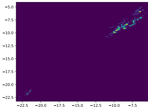
Figure 3: The distribution of the estimated Fisher diagonals shown in heat map, with x-axis for the means of the log squared gradients of each weight or bias, and y-axis the standard deviation.
