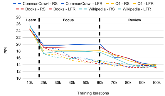
Figure 5: PPL values are tracked at different training iterations for the clusters identified as easy, discarded during the Focus stage, and reintroduced during the Review phase. The dotted line represents the PPL values for the same clusters when trained with random sampling (RS). Notably, we demonstrate that models forget the data points discarded during training, unless reintroduced to the training corpus as in the case of LFR.
