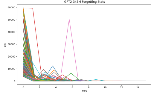
Figure 3: PPLs of data samples being forgotten by the GPT2-345M model. This multi-descent behavior is exhibited by 20% of the data.
