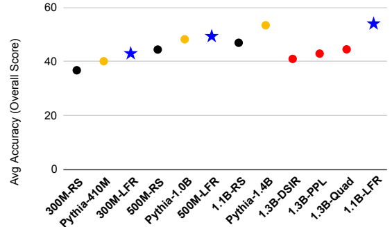
Figure 1: Average accuracy norm across common-sense reasoning, problem-solving, world knowledge, and reading comprehension tasks. Across model sizes (300M–1.1B), LFR (stars) outperforms full-dataset training (RS in black circles) by 6%, Pythia (yellow circles) by 1.5%, and Quad (Zhang et al., 2024) (red circle) by 9%, using only 3–6% and 65% of the training tokens of Pythia and Quad, respectively. Notably, Pythia and Quad have larger parameter counts. See Section 5 for details.
