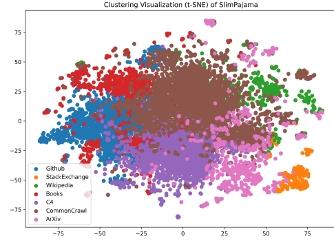
Figure 6: Clustering the data embeddings from the SlimPajama dataset using the Llama-300M model at the 50k training step.
