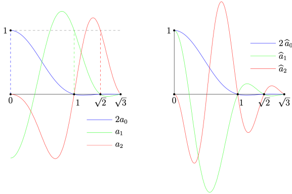
Fig. 1. Plots of the first few a_n, \hat{a}_n taken from [4]. Note that \hat{a}_0 = a_0 .
