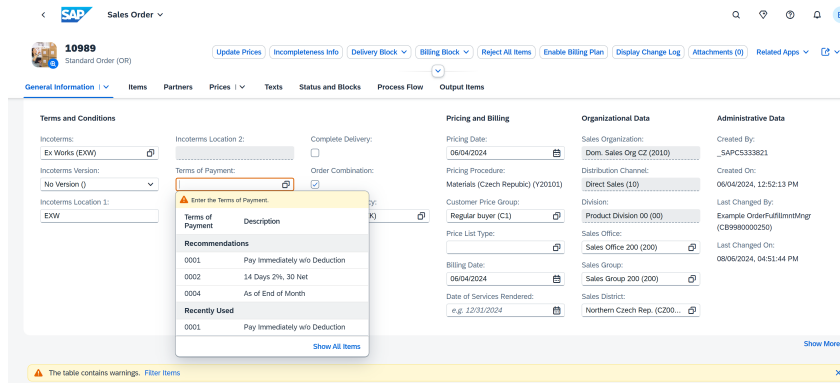
Figure 5: Illustrative example of a real-world autocomplete task, where the SAP S/4HANA Sales Order User interface (Klein et al., 2024) predicts payment terms based on other filled-in response fields.
