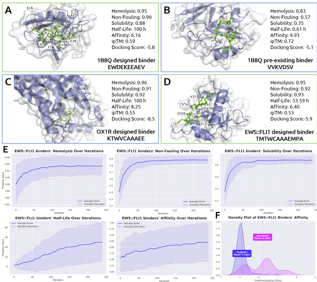
Figure 1: (A), (B) Complex structures of PDB 1B8Q with an AREURDi-designed binder and its pre-existing binder. (C), (D) Complex structures of OX1R and EWS::FL1I with an AREURDi-designed binder. Five property scores are shown for each binder, along with the ipTM score from AlphaFold3 and docking score from AutoDock VINA. Interacting residues on the target are visualized. (E) Plots showing the mean scores for each property across the number of iterations during AREURDi’s design of binders of length 12-aa for EWS::FL1I. (F) A density plot illustrating the distribution of predicted property scores for AREURDi-designed EWS::FL1I binders of length 12-aa, compared to the peptides generated unconditionally by PepReDi 3 .
