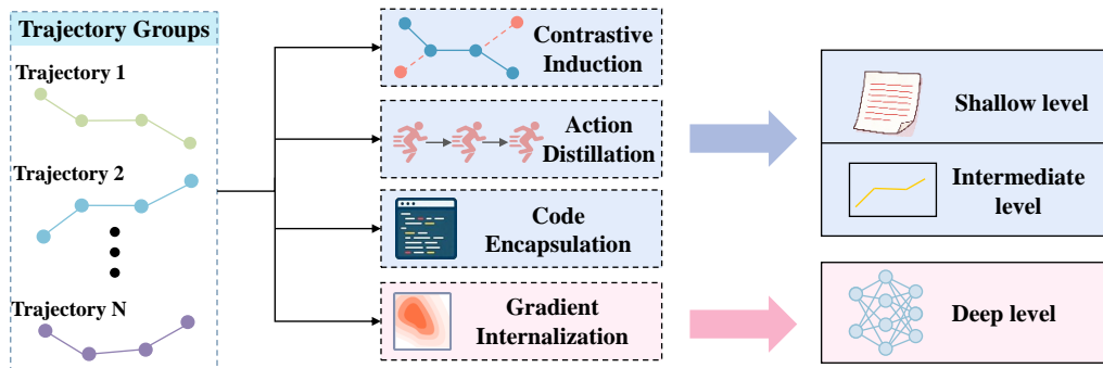
Figure 3: Overview of Cross-Trajectory Abstraction.
