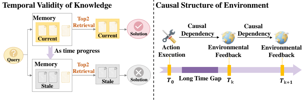
Figure 2: The Drivers in Dynamic Environments.
