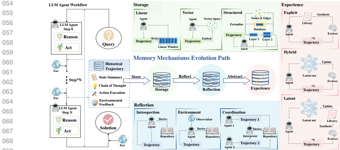
Figure 1: Overview of the LLM agent Memory Mechanisms System.
