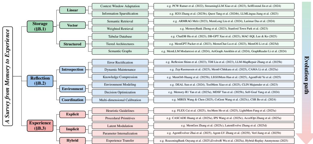
Figure 4: Taxonomy of LLM agent Memory Mechanisms
