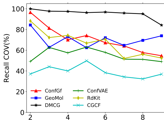
Figure 4: Coverage scores w.r.t. number of rotatable bonds.
