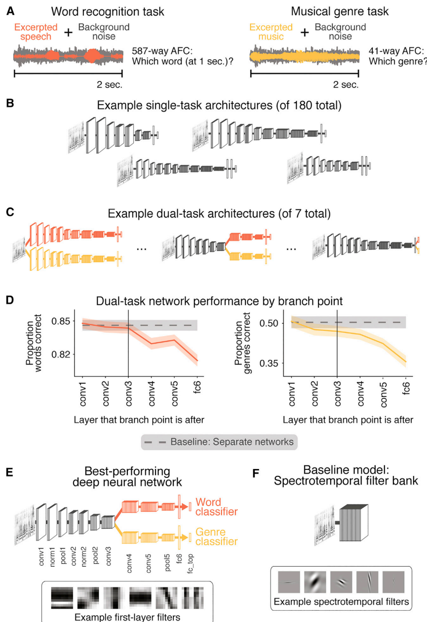
Figure 1. Deep Neural Network Training: Tasks and Architecture Search
