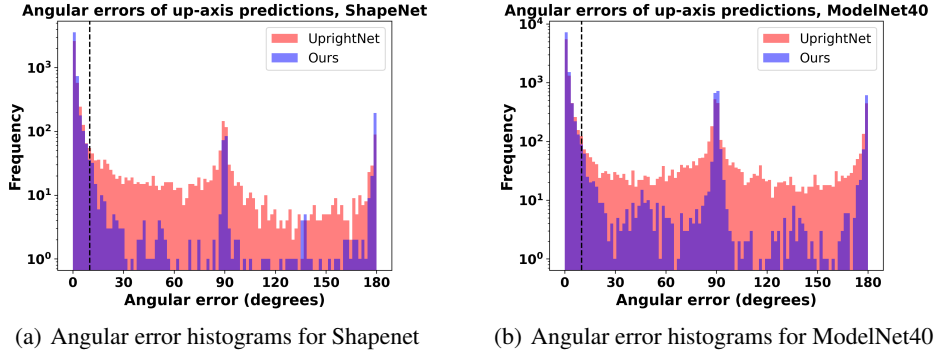
Figure 6: Comparison of angular errors between the estimated and ground truth up-axis on the Shapenet validation set (left) and on ModelNet40 (right). Frequencies are plotted in log scale. The dashed lines indicate the 10^\circ error threshold beyond which a prediction is treated as incorrect. Our algorithm’s error rate is 64.6% lower than the prior state of the art.
