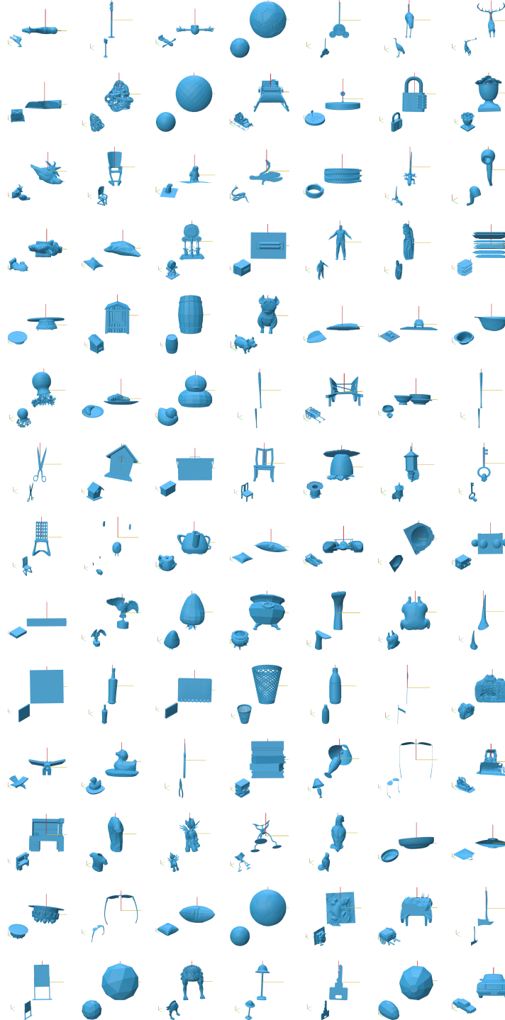
Figure 11: A grid of our model’s top-1 outputs given randomly rotated, non-cherrypicked meshes from Objaverse. We depict a front view of our model’s recovered shapes along with an inset depicting an isometric view. Our quotient regressor consistently succeeds on out of distribution meshes, as most of our pipeline’s outputs are correctly oriented up to a cube flip. Our flipper has greater difficulty generalizing, but predicts an acceptable flip in many cases. We expect that training on a larger and more diverse dataset of oriented shapes will improve our flipper’s generalization performance.
