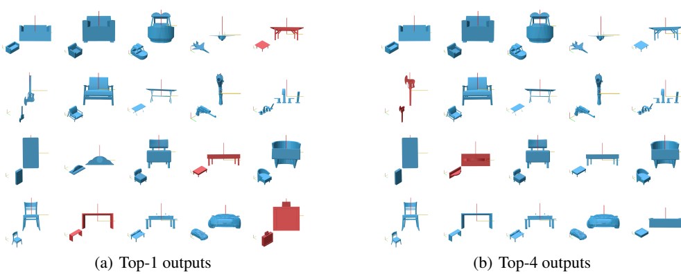
Figure 8: Comparison of oriented shapes recovered using the flipper’s highest-probability flip (left) and the best flip among the top 4 classes in the flipper’s model distribution (right). Our pipeline correctly infers the full orientation of most shapes, and many of its failures correspond to orientations that are acceptable in practice.
