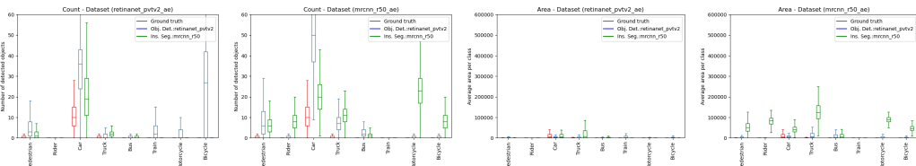
Figure 17: OD_retinanet_pvtv2_SEG_mrcnn_r50
