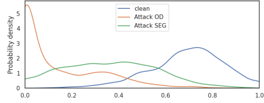
Figure 51: OD_retinanet_pvtv2_SEG_mask2former
