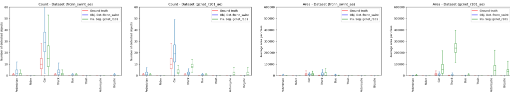
Figure 16: OD_frnn_swint_SEG_gcnct_r101
