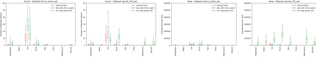
Figure 13: OD_frnn_swint_SEG_gcnct_r50
