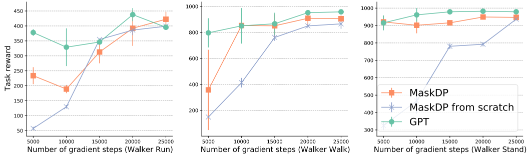
Figure 8: Offline RL results on Walker domain. The result of MaskDP matches the GPT-style pretraining performance, and are all comparable to the SoTA in ExoRL [37].
