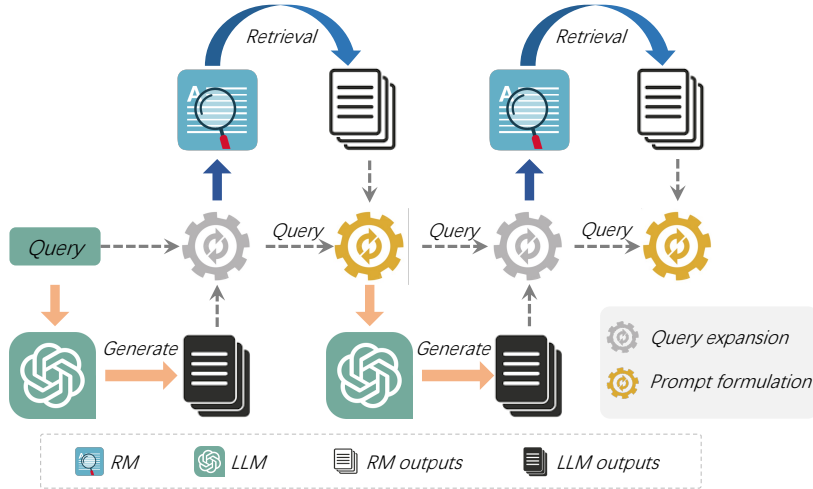
Figure 1: Overall architecture of InteR.
