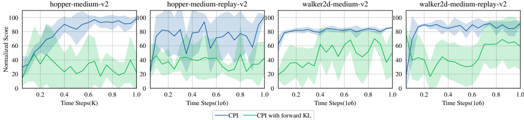
Figure 9: Effect of using different KL strategies. Reverse KL-based CPI exhibits superior performance compared to the forward KL-based CPI. See Appendix for details of forward KL.
