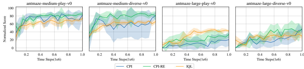
Figure 7: The learning curves of CPI, CPI-RE, and IQL on Antmaze. With reference ensemble, CPI-RE exhibits a more stable performance compared to vanilla CPI, also outperforming IQL.
