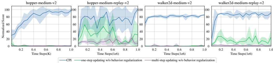
Figure 8: Effect of using Behavior Regularization. Without it, both one-step and multi-step updating methods at each gradient step suffer from deviation derived from out-of-support optimization.
