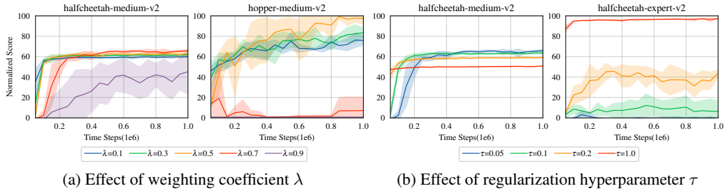
Figure 10: Hyperparameters ablation studies. The tuning experience drawn from this include: (1) \lambda could mostly be set to 0.5 or 0.7; (2) The higher the dataset quality is, the higher \tau should be set.
