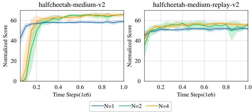
Figure 11: Effect of different actor number
