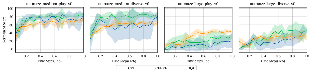
Figure 3: The learning curves of CPI, CPI-RE, and IQL on Antmaze. With reference ensemble, CPI-RE exhibits a more stable performance compared to vanilla CPI, also outperforming IQL.
