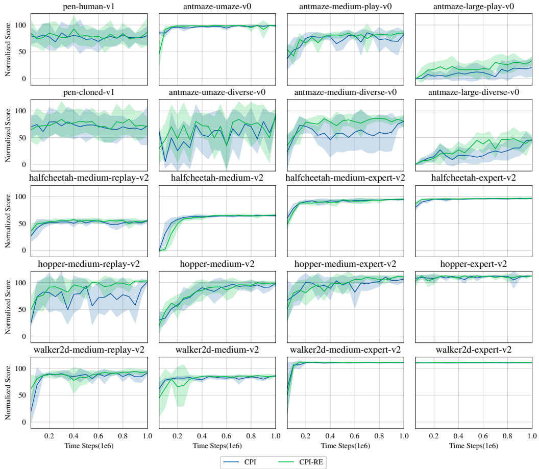
Figure 12: Learning curves of CPI and CPI-RE for Mujoco, Antmaze and Pen, evaluated every 5e3 steps.
