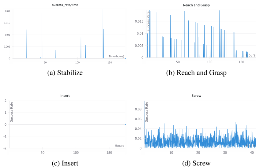
Figure A.13: Learning curves for RL with point-cloud observations and joint position actions.
