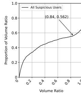
Figure 7: CDF of volume ratios for per user.
