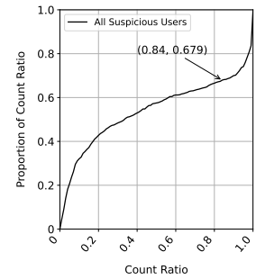
Figure 8: CDF of count ratios for per user.
