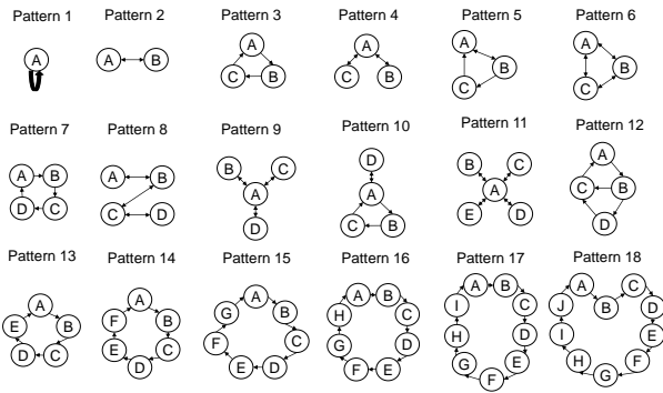
Figure 9: Summary of wash trading patterns.
