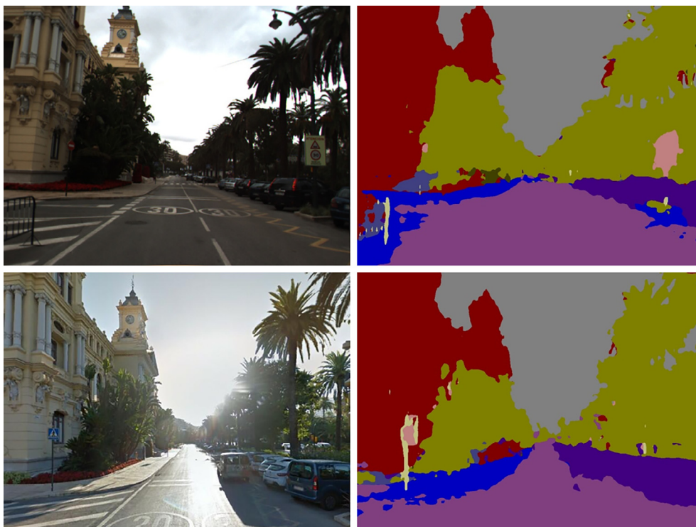
Fig. 2. On the left, two images of the same scene with considerable illumination changes. On the right, their semantic segmentation results. Standard methods have low performance for such cases, where more stable semantic segmentation can help.
