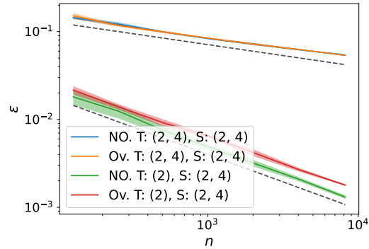
Figure S5: Learning curves for deep convolutional NTKs ( \nu = 1/2 ) with non-overlapping (NO.) and overlapping (Ov.) patches in a teacher-student setting with inputs normalised in the d -hypercube. The numbers inside brackets are the sequence of filter sizes of the kernels. Solid lines are the results of experiments averaged over 16 realisations with the shaded areas representing the empirical standard deviations. The asymptotic scaling \epsilon \sim n^{-\beta} predicted for kernels with non-overlapping patches are reported as dashed lines.
