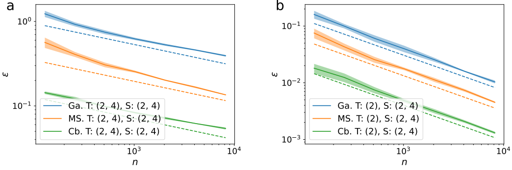
Figure S4: Learning curves for deep convolutional NTKs ( \nu = 1/2 ) in a teacher-student setting with different input normalisations. In particular, we consider inputs on the multisphere M^p S^{s-1} (MS.), uniformly-distributed in the unit d -hypercube [0, 1]^d (Cb.), and with standard Gaussian distribution \mathcal{N}(0, I_d) (Ga.). The numbers inside brackets are the sequence of filter sizes of the kernels. Solid lines are the results of experiments averaged over 16 realisations with the shaded areas representing the empirical standard deviations. The asymptotic scaling \epsilon \sim n^{-\beta} predicted for inputs on the multisphere are reported as dashed lines.
