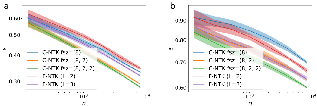
Figure S6: Learning curves of the neural tangent kernels of fully-connected (F-NTK) and convolutional (C-NTK) networks with various depths learning to classify two CIFAR-10 classes in a regression setting. Deep hierarchical convolutional kernels achieve the best performance. Shaded areas represent the empirical standard deviations obtained averaging over different training sets. a. Plane vs car. b. Cat vs bird.
