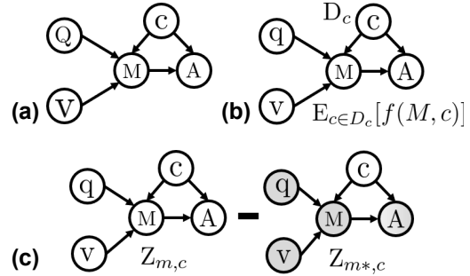
Figure 2: Demonstration of (a) our proposed causal graph for multimodal tasks, (b) Average Treatment Effect (ATE), and (c) Total Effect (TE) on (a). Values in grey indicate the ‘no-treatment’ condition.
