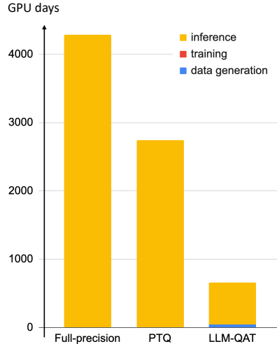
Figure 4: Total computation cost over 5 million inferences.
