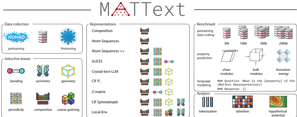
Figure 1: Overview of the MatText framework. For MatText, we compile pretraining and fine-tuning data and implement text representations of crystal structures with different inductive biases in a standardized, object-oriented framework. We use the data and text representations to build a property-prediction benchmark for language modeling of materials properties and analyze the models and results to reveal the limitations of current approaches.
