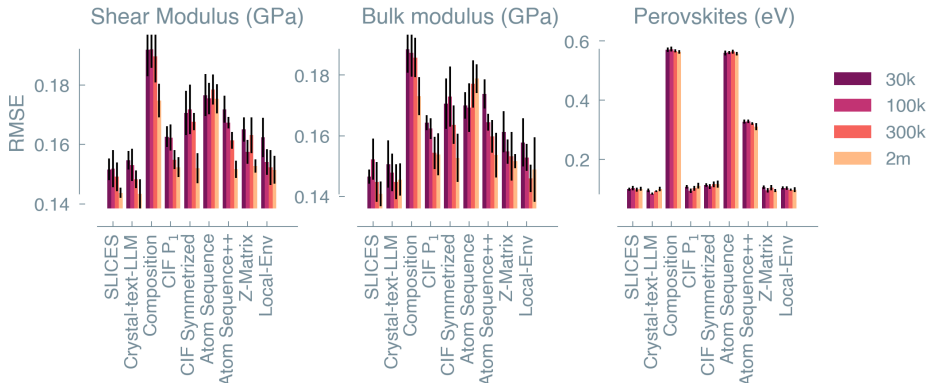
Figure 2: MatText-BERT scaling cross-validation scores. We pretrained BERT models with increasing pretraining dataset sizes (indicated in color) and fine-tuned them for material property prediction tasks using different material text representations. The error bars indicate the standard deviation across cross-validation folds.
