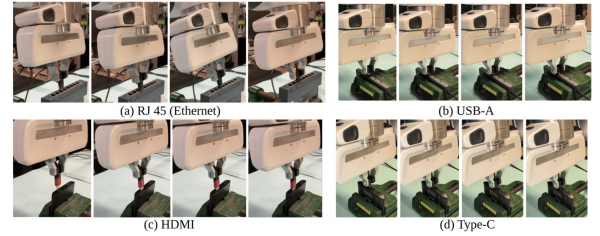
Fig. 2. Four typical electronic component assembly tasks: RJ45 (polygonal), USB-A (rectangular), HDMI (trapezoidal), and Type-C (oval) connectors with 0.1-0.2 mm assembly tolerances. The high precision of the assembly tolerances and different sizes require compliance control of pose and wrenches, with experimental validation video in the supplement.
