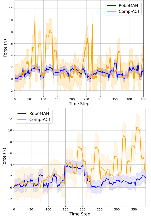
Fig. 3. Comparative analysis of assembly contact forces. Top: The contact force measured during Type-C assembly with RoboMAN and Comp-ACT. Bottom: Comparison of contact force between RoboMAN and Comp-ACT during the transition between variable assembly tasks. The transition occurs at approximately the 150th time step and ends around the 210th step.
