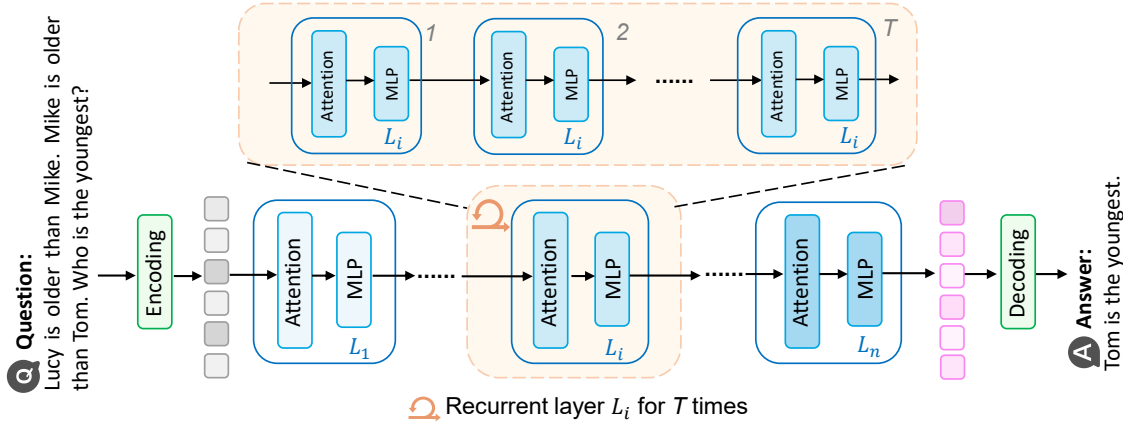
Figure 6: Simplified illustration of layer-recurrent execution for implicit reasoning, which usually reuses the same parameters at recurrent layers (or blocks) to refine reasoning through depth-wise computation.
