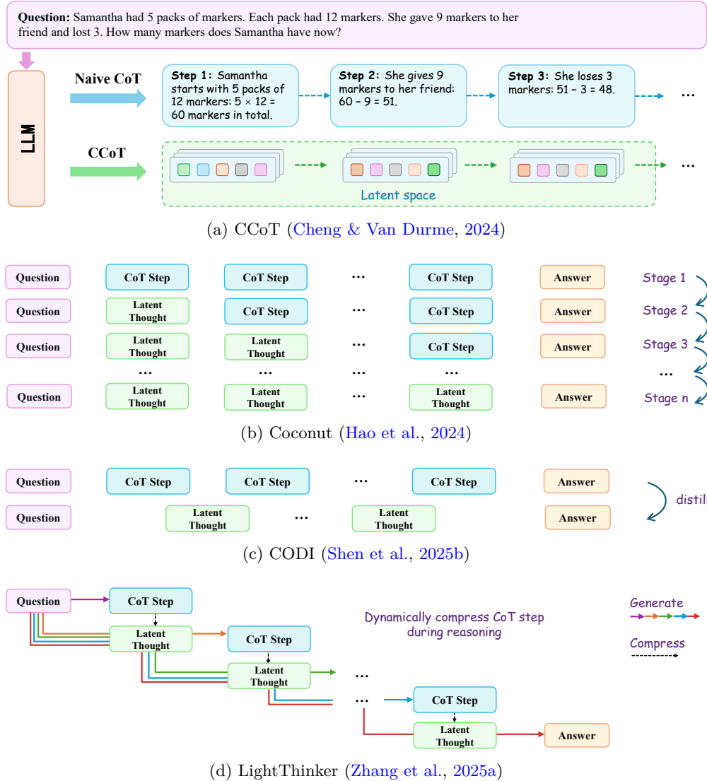
Figure 4: Trajectory-level latent optimization. Illustration of representative methods for encoding multi-step reasoning trajectories in latent space: (a) CCoT compresses the full CoT traces into short sequences of continuous embeddings, reducing decoding cost while preserving essential reasoning semantics (Cheng & Van Durme, 2024). (b) Coconut replaces discrete reasoning steps with latent thoughts in a multi-stage training process, enabling latent reasoning progressively (Hao et al., 2024). (c) CODI distills explicit CoTs into continuous latent thoughts under a self-distillation framework in a single-stage compression manner (Shen et al., 2025b). (d) LightThinker (Zhang et al., 2025a) dynamically compresses reasoning steps into latent gist tokens at the designated position, reducing memory and computational overhead.
