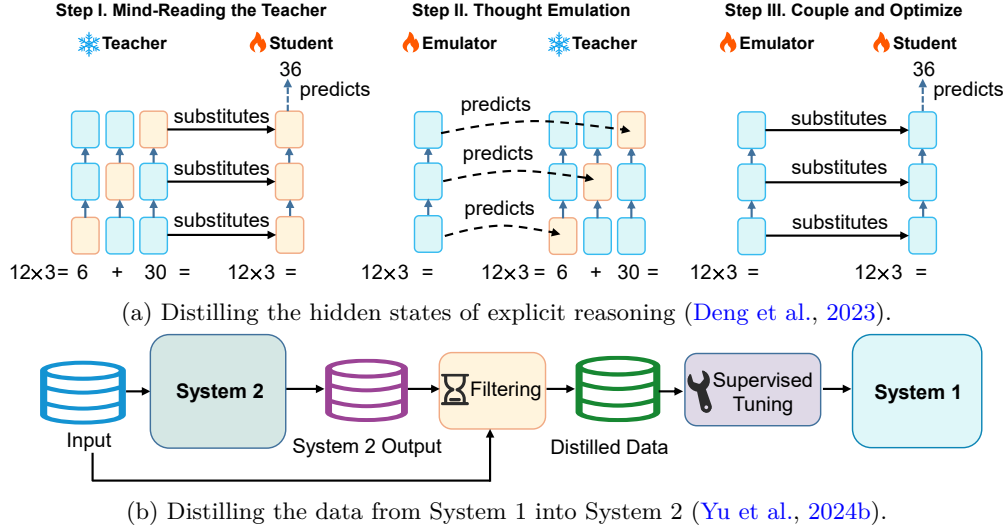
Figure 5: Two representative distillation methods of internal-state-level latent optimization.
