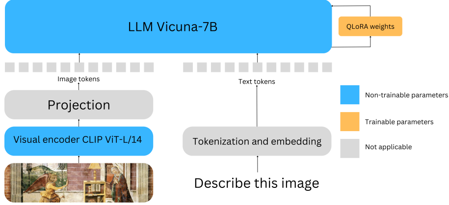
Figure 1: Architecture of LLAVA model with QLoRA layer
