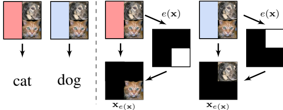
Figure 3: Left: Consider data where the color in the left half determines whether the label (“cat”, “dog”) is produced from the top or bottom image on the right. Right: A MARG encoding explanation that produces only the top or the bottom animal image based on the color. The animal image alone says less about the label than knowing the animal image and the color. Knowing the selection determines the color and thus provides additional information about the label.
