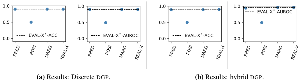
Figure 6: The EVAL-X-ACC and AUROC scores for the different explanations for the discrete DGP are on the left and the scores for the hybrid DGP are on the right. In both, multiple encoding explanations (PRED, MARG, and the reductive one from REAL-X) all achieve the same score as the corresponding EVAL-X* score. Thus, ranking metrics like accuracy and AUROC are not sensitive to encoding explanations like EVAL-X log-likelihoods, and can fail to even weakly detect encoding. This stems from the fact that accuracy and AUROC only depend on the ranking of the datapoint, and therefore are not sensitive to differences in log probabilities that do not change ranks.
