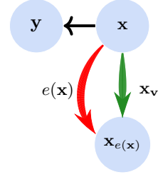
Figure 2: Intuition for encoding: There are two ways the information in the inputs \mathbf{x} about the label \mathbf{y} is transmitted to the explanation \mathbf{x}_{e(\mathbf{x})} : 1) through the values in the explanation and 2) the selection e(\mathbf{x}) (red arrow). When the latter happens, the explanation is said to be encoding .
