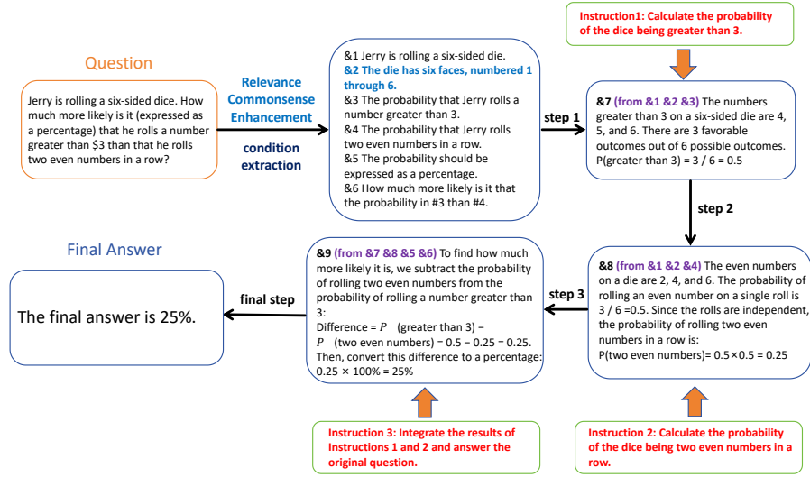
Figure 1: An example of Commonsense-Augmented Progressive Instruction Reasoning
