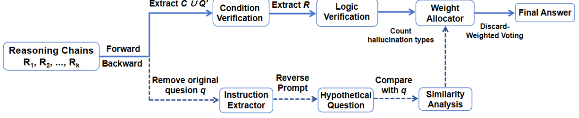
Figure 2: Architecture of Multi-Dimensional Heterogeneous Collaborative Verification
