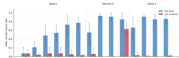
Figure 14. Peak corrupt rhyme rate (maximum across all layers) for the last word token and newline ( i = 0 ) at each model size. Black error bars are 95% cluster bootstrap CIs over prompt pairs (5 pairs per model). Gemma-3-27B is the only model whose newline CI is clearly separated from zero (0.63 [0.48, 0.78]); every other model has a newline CI upper bound \leq 0.21 regardless of scale, while last-word patching is broadly effective from \sim 3 B parameters onward in every family.
