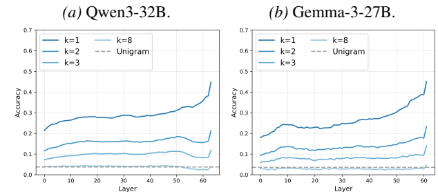
Figure 11. Top-1 probe accuracy predicting k tokens ahead in general text (Pile). Mirrors the top-5 pattern: accuracy degrades monotonically with k and falls to unigram baseline by k = 8 .
