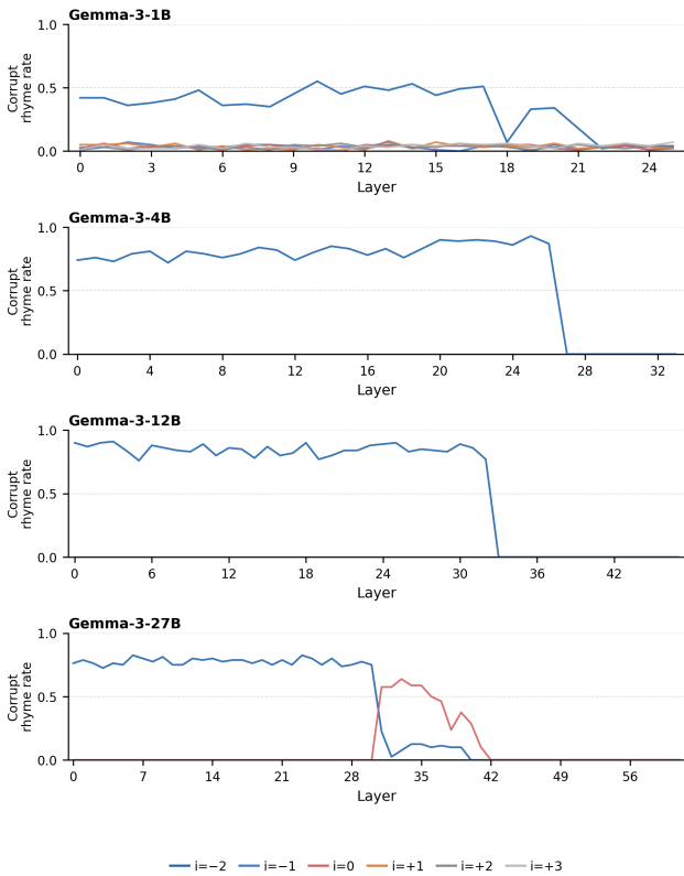
(c) Gemma-3 1B–27B.
