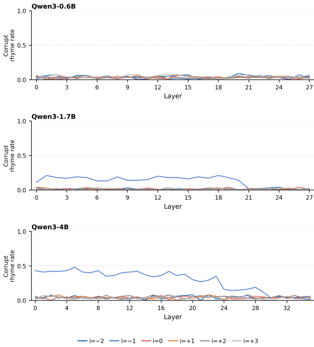
(a) Qwen3 0.6B–4B.
