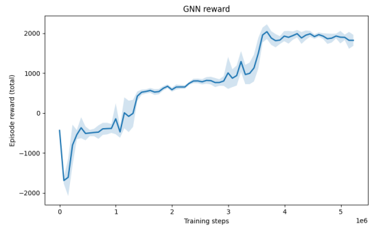
Fig. 5. Evaluation rewards of GNN policy during training.
