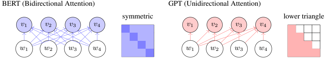
Figure 2: Illustration of Attention Relationships in BERT and GPT with Corresponding Attention Matrix Representations
