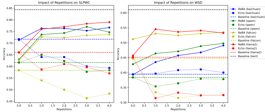
Figure 3: Word Embeddings : Performance on SLPWC and WSD tasks using Euclidean distances to evaluate Word Embeddings . The results show that ReBA encoding significantly enhances model performance on polysemous word understanding tasks. While performance fluctuates with the number of repetitions, increasing the repetition count does not necessarily lead to significant improvements. Based on this experiment, we observe that simple sentence repetition is not effective for improving word-level embeddings and only contributes to sentence-level understanding. Furthermore, the backward attention mechanism remains crucial for achieving further performance enhancements.
