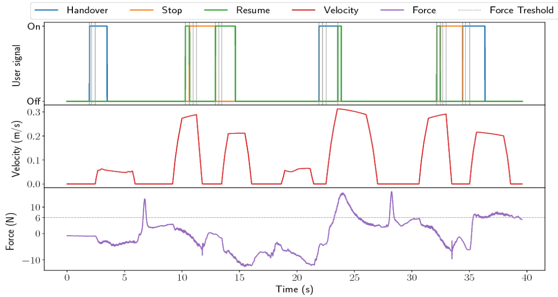
Fig. 9. Illustration of detected user inputs (top), l2-norm of end-effector velocity (center) and l2-norm of force applied on the end-effector (bottom).
