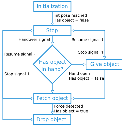
Fig. 7. Finite state machine of the robotic handover experiment.
