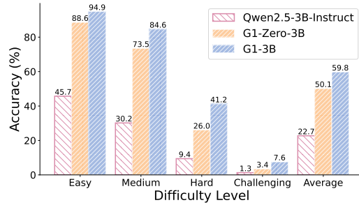
Figure 1: Test accuracy comparison of G1-3B and G1-Zero-3B on our benchmark. We include results for -7B in Appendix H.1.
