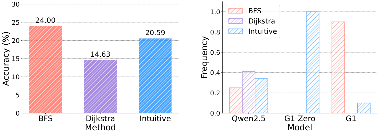
(a) The accuracy of different graph reasoning patterns for shortest path on Qwen2.5-3B-Instruct.
