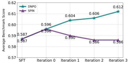
Figure 5: Average scores across iterations show DNPO consistently improving, while SPIN stagnates after the first iteration.
