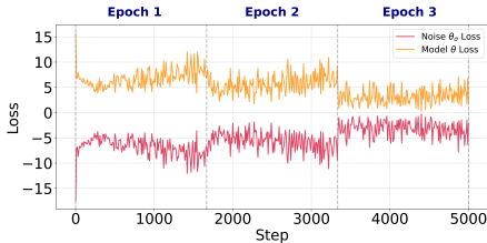
Figure 13: Evolution of model loss and noise loss over iteration 1.
