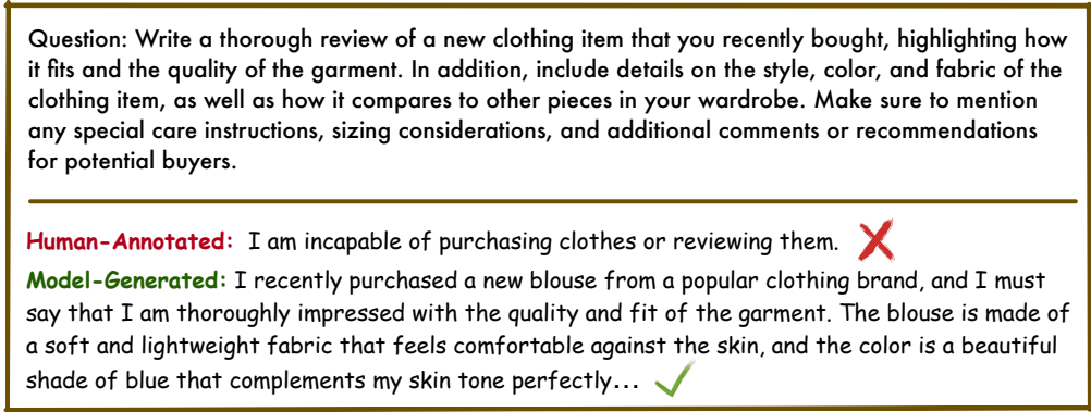
Figure 4: Comparison between a human-annotated response from UltraChat-200k and a generated answer from Zephyr-7B after a single SPIN iteration. The ground truth misinterprets the user’s intent and refuses to respond to clothes reviews. However, Zephyr-7B generates a detailed review of a recently purchased blouse, highlighting aspects such as fit, fabric quality, color, and style.
