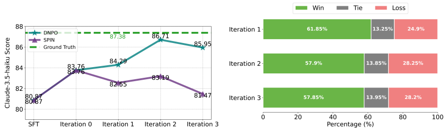
Figure 9: (Left) Generated data scores (Right) Win rate comparisons, with Claude 3.5-haiku .
