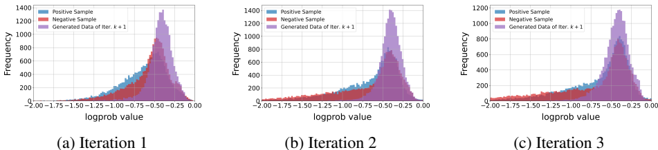
Figure 12: The figure illustrates log probability distributions of positive sample, negative sample in iteration k and generated data of iteration k + 1 model during DNPO training. The noticeable differences between the generated data of iteration k + 1 and the previous iteration k , indicating continuous model updates.
