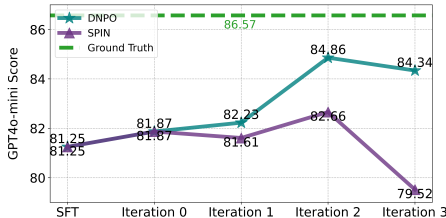
Figure 6: Average GPT4o-mini scores across iterations for generated data of DNPO and SPIN, alongside ground truth.
