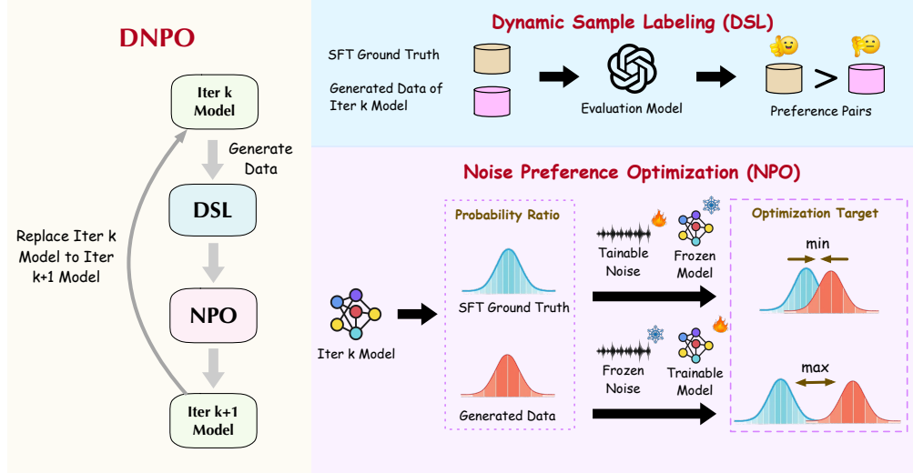
Figure 3: This diagram illustrates the iterative training process of DNPO. There are two core components: Dynamic Sample Labeling (DSL) and Noise Preference Optimization (NPO).
