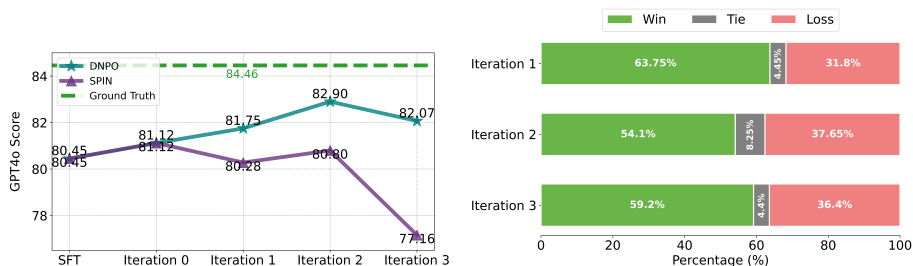
Figure 10: (Left) Generated data scores (Right) Win rate comparisons, with GPT4o .
