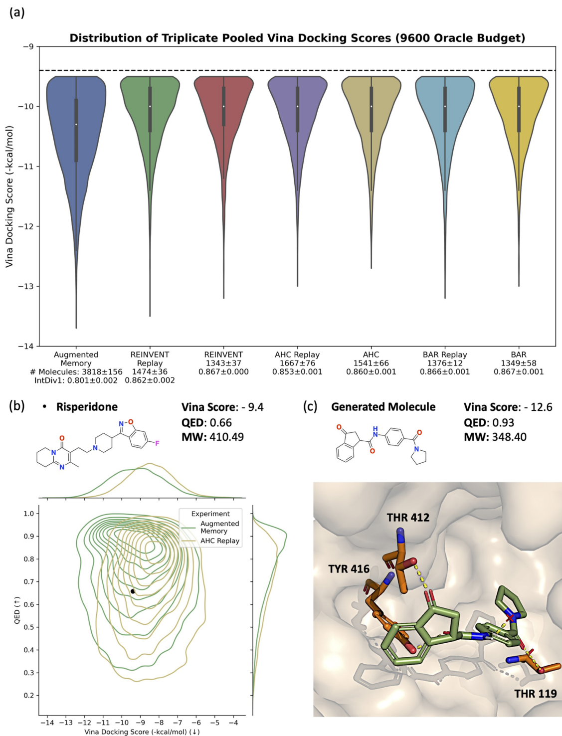
Figure 4. DRD2 case study. PDB ID: 6CM4. (a) Docking score distribution of all compared algorithms. (b) Augmented Memory jointly optimizes QED-Vina score, demonstrating the ability to perform MPO. (c) Binding pose of a generated molecule using Augmented Memory. The three components in the objective function: MW < 500, QED, and Vina docking score are all optimized.
