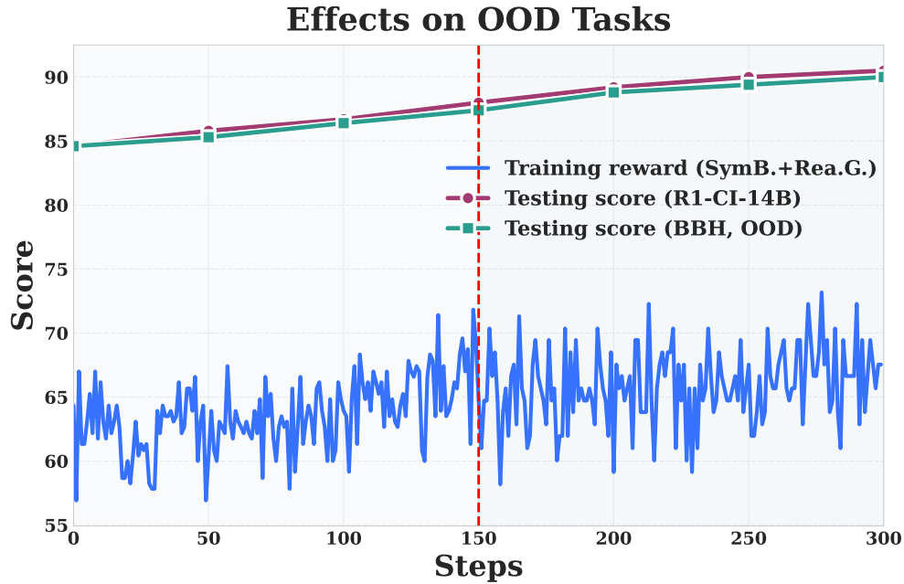
Figure 13: Evaluation on out-of-distribution (OOD) tasks. We trained the 14B model using two-stage GRPO with SymbBench and Reasoning-Gym as training data, and evaluated it on Big-Bench-Hard(BBH) as an OOD benchmark. The number of training tasks remained 107. The blue curve shows the steadily increasing reward during two-stage GRPO training. Comparing the BBH test results of the new model (green curve) with the original R1-CI-14B model (purple curve) shows similar performance, indicating that our training framework generalizes effectively to unseen task distributions from varied sources.
