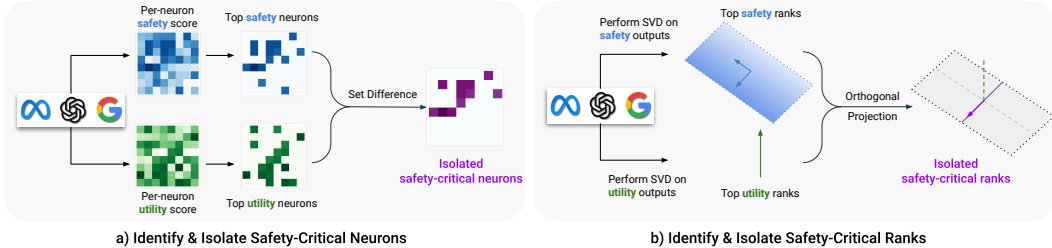
Figure 1: The proposed pipelines for identifying and isolating safety-critical regions of LLM weights at (a) neuron level and (b) rank level.
