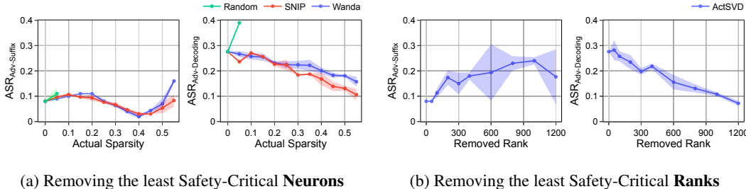
Figure 3: Impact on ASR under adversaries in Llama2-7B-chat when: (a) Removing neurons with the lowest safety importance scores and (b) Removing the least safety-critical ranks identified by ActSVD. Both the importance score and safety-critical ranks are calculated on the safety-short dataset. All plotted points have reasonable utility with accuracy > 0.5 . The exclusion of neurons and ranks deemed least critical for safety results in improved robustness against adversarial decoding attacks. Potential reason for the variation in \text{ASR}_{\text{Adv-Suffix}} is the adversarial suffixes may not directly transfer to the modified model. See Figure 6 for the results on Llama2-13B-chat.
