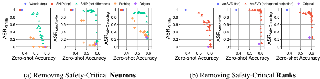
Figure 2: ASR and accuracy after removing safety-critical neurons with sparsity constraint < 3\% (a) and ranks with ranks of the weight updates ( \text{rank}(\Delta W) ) less than 100 (b) in Llama2-7B-chat. Disentangling safety from utility (set difference for neurons and orthogonal projection for ranks) mostly effectively identify the safety-critical regions, with safety severely compromised while utility retains.
