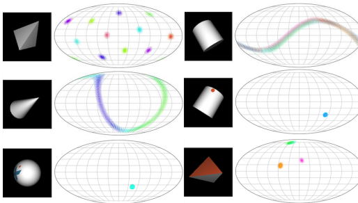
Figure 6: Visualization of pose distribution on SYMSOL . The results are obtained by joint training with both our regression loss and the cross-entropy distribution loss [35, 49].
