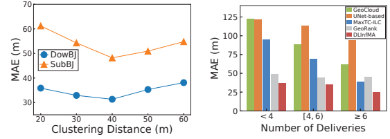
(a) Distance Selection. (b) Different #Deliveries.
