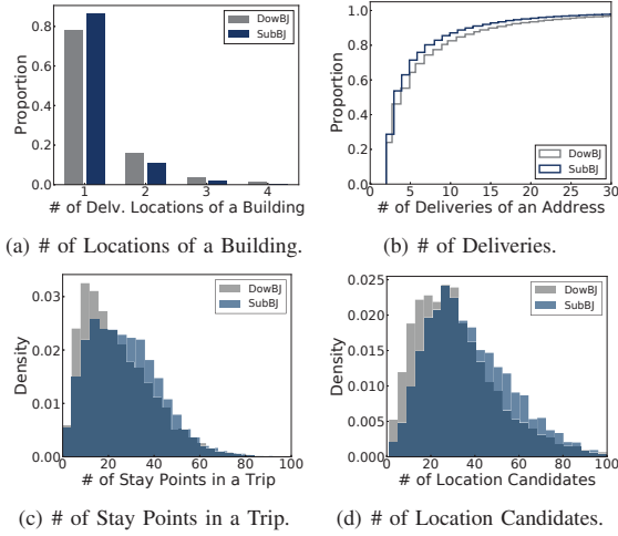
Fig. 9. Dataset Descriptions.
