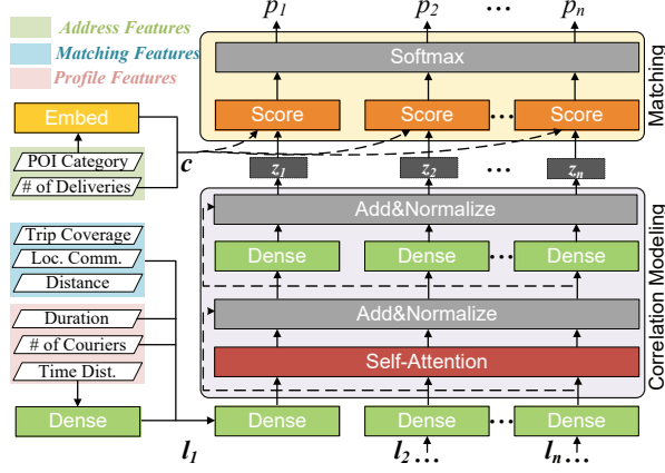
Fig. 8. LocMatcher Architecture.
