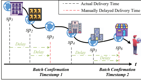
Fig. 11. Illustration of Generating Synthetic Datasets.
