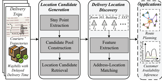
Fig. 3. Framework of DLInfMA.
