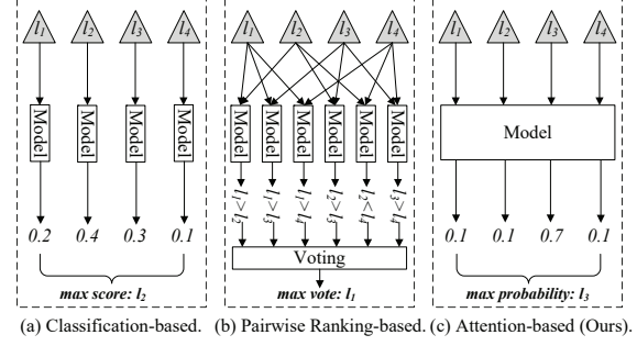
Fig. 7. Different Location Selection Strategies.
