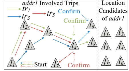
Fig. 5. Illustration of Location Candidate Retrieval.
