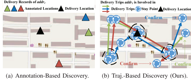
Fig. 2. Annotation-Based V.S. Trajectory-Based Discovery.
