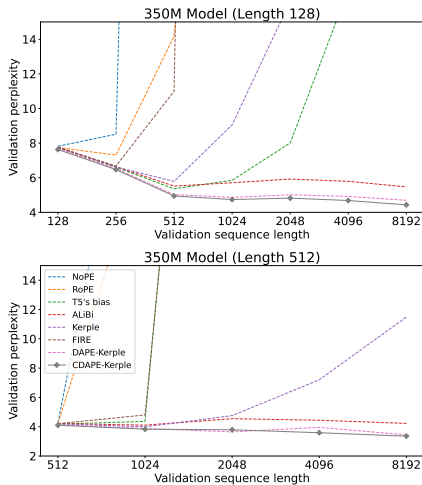
Figure 4: The Effect of Larger Model Size 350M. We show the results with training length 128 and training length 512 on Arxiv dataset.
