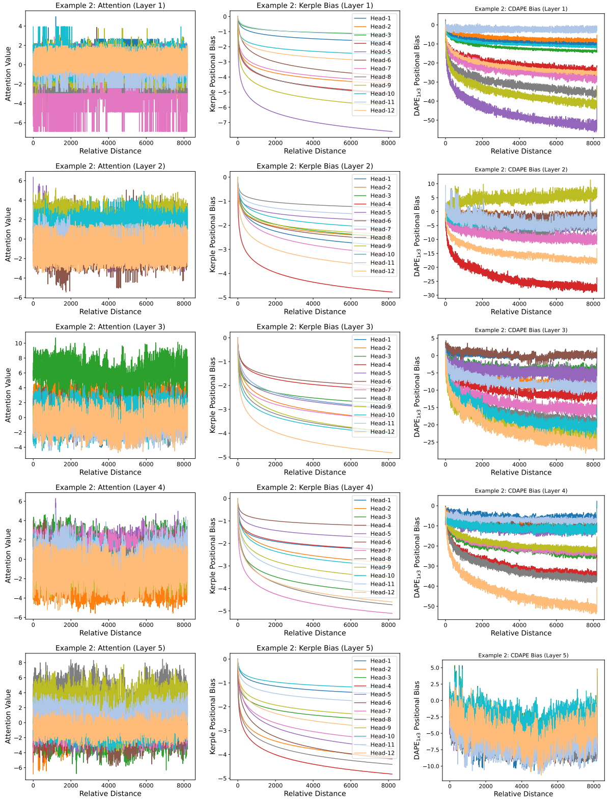
Figure 23: Evaluation Length 8192 Example 2: Part 1. From Left to Right: (1) The Attention is XW_Q(XW_K)^\top ; (2) The Kerple bias is B ; (3) The CDAPE (with Kerple) bias is f(XW_Q(XW_K)^\top, B) .
