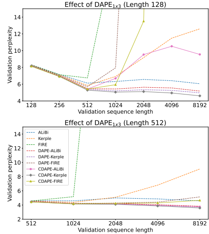
Figure 5: The effect of CDAPE. Whatever the baseline is ALiBi, Kerple or FIRE, the proposed CDAPE can all improve their performance. The Figure 1 also proves that the proposed CDAPE is effective for NoPE and RoPE.
