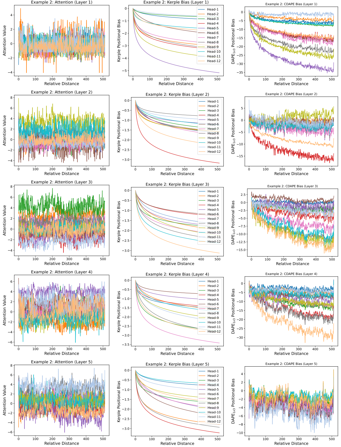
Figure 11: Evaluation Length 512 Example 2: Part 1. From Left to Right: (1) The Attention is XW_Q(XW_K)^\top ; (2) The Kerple bias is B ; (3) The CDAPE (with Kerple) bias is f(XW_Q(XW_K)^\top, B) .
