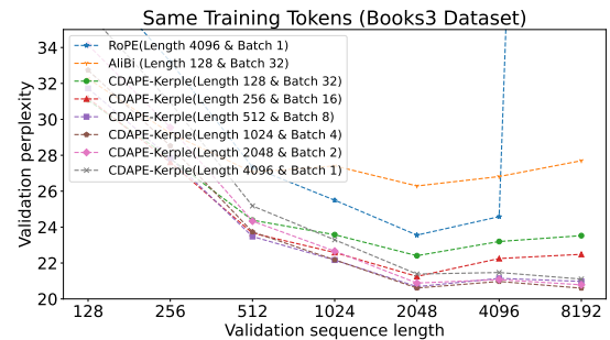
Figure 3: The performance with same training tokens and different training length. With the same training tokens, CDAPE with training length 512 could even achieve better performance than RoPE with training length 4096.
