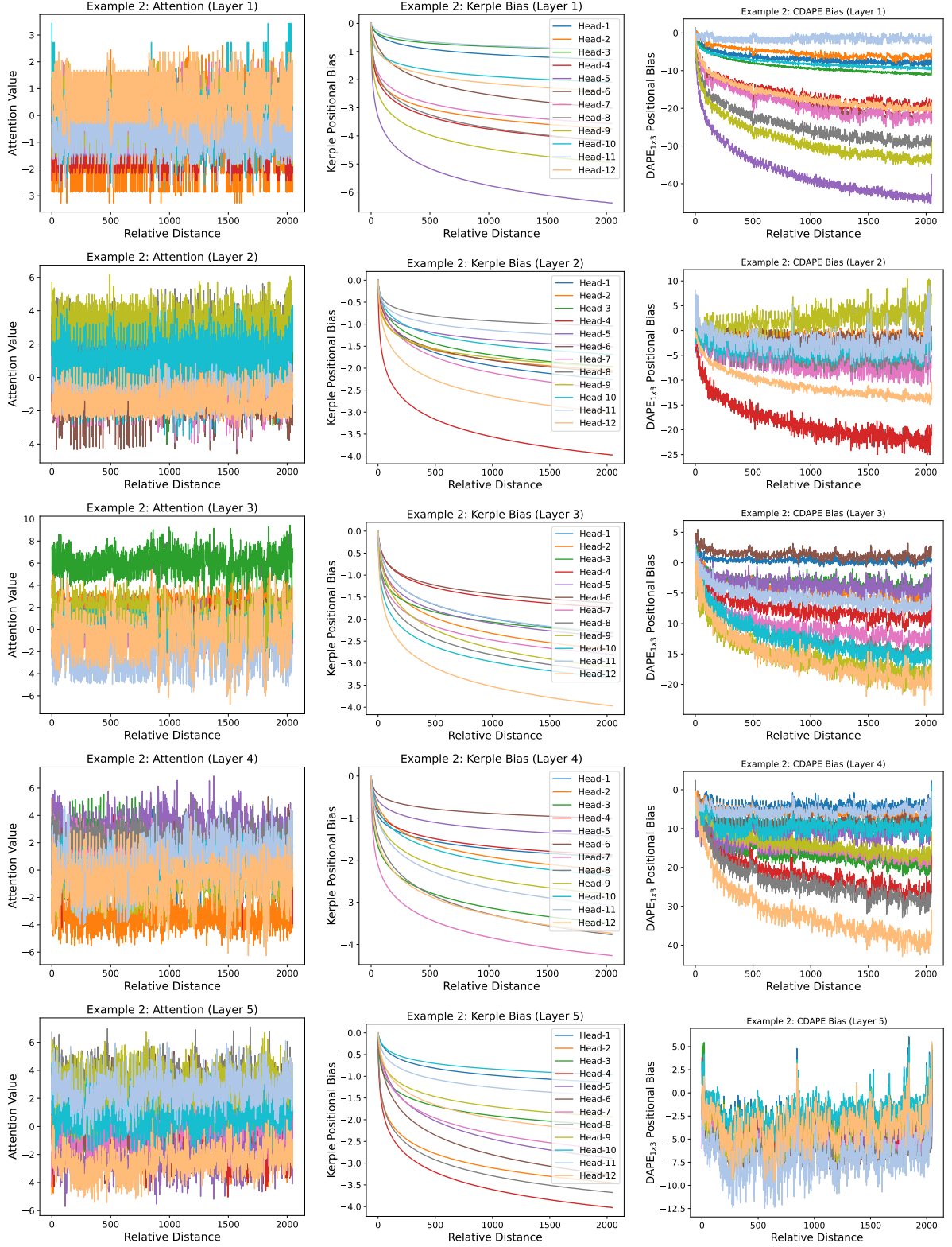
Figure 17: Evaluation Length 2048 Example 2: Part 1. From Left to Right: (1) The Attention is XW_Q(XW_K)^\top ; (2) The Kerple bias is B ; (3) The CDAPE (with Kerple) bias is f(XW_Q(XW_K)^\top, B) .
