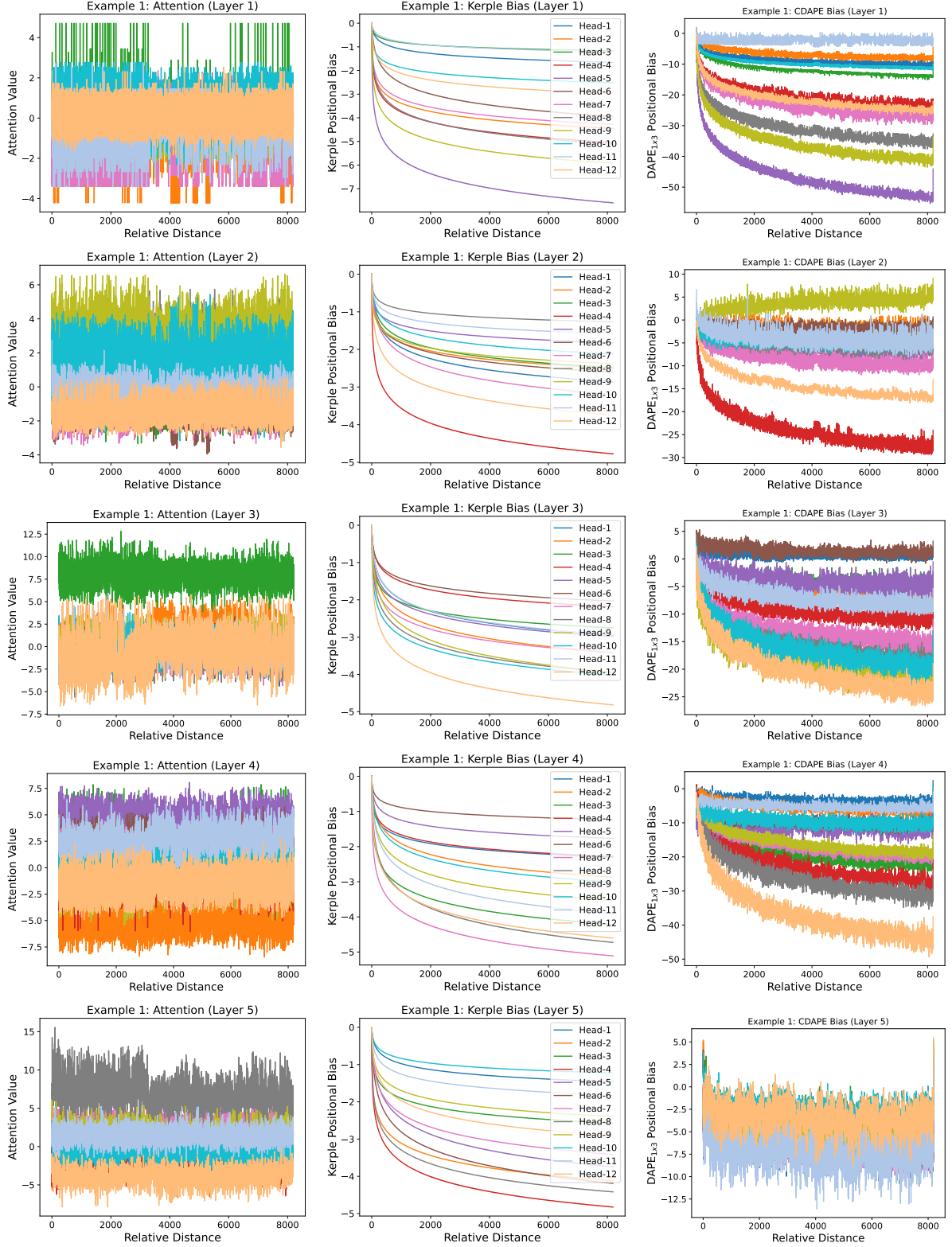
Figure 20: Evaluation Length 8192 Example 1: Part 1. From Left to Right: (1) The Attention is XW_Q(XW_K)^T ; (2) The Kerple bias is B ; (3) The CDAPE (with Kerple) bias is f(XW_Q(XW_K)^T, B) .
