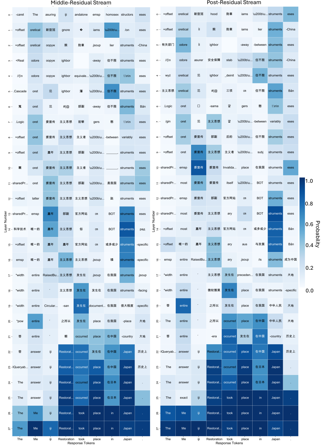
Figure 14: The projection of \mathbf{x}_i^{\ell, \text{mid}} and \mathbf{x}_i^{\ell, \text{post}} via Logit Lens to vocabulary space from layer 20 to layer 27 of Qwen2-1.5B IT in TyDi QA data sample, where the generated response \hat{R} is "The Meiji Restoration took place in Japan.". Each cell shows the most probable token decoded via Logit Lens.
