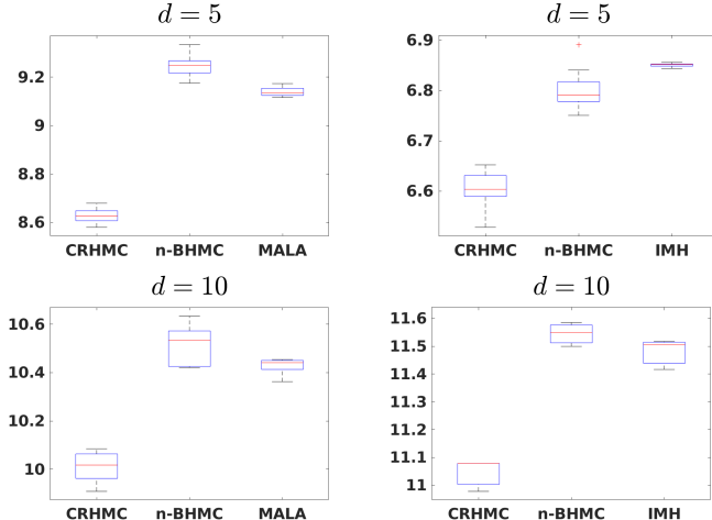
Figure 2: Comparison between n-BHMC and CRHMC on the hypercube (left) and the simplex (right).
