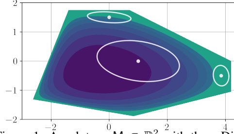
Figure 1: A polytope M \subset \mathbb{R}^2 with three Dikin ellipsoids \{y \in \mathbb{R}^d : y^\top \mathbf{g}(x)y < 1\} derived from its logarithmic barrier.
