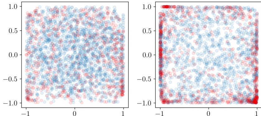
Figure 3: Outputs of n-BHMC after 25k iterations to sample from the uniform distribution over [-1, 1]^2 with \eta = 10^{-3} , h = 0.8 , using in (8) the “self-concordant” norm (left) or the Euclidean norm (right). Red samples are rejected and blue samples are accepted.
