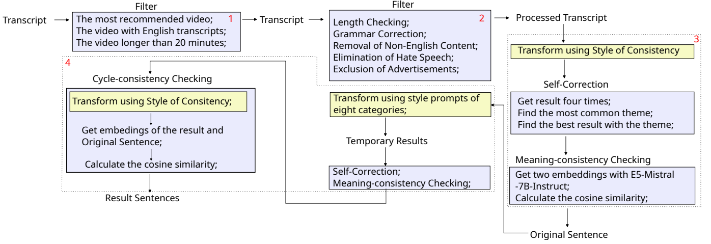
Fig. 1: The Workflow of Data Generation
