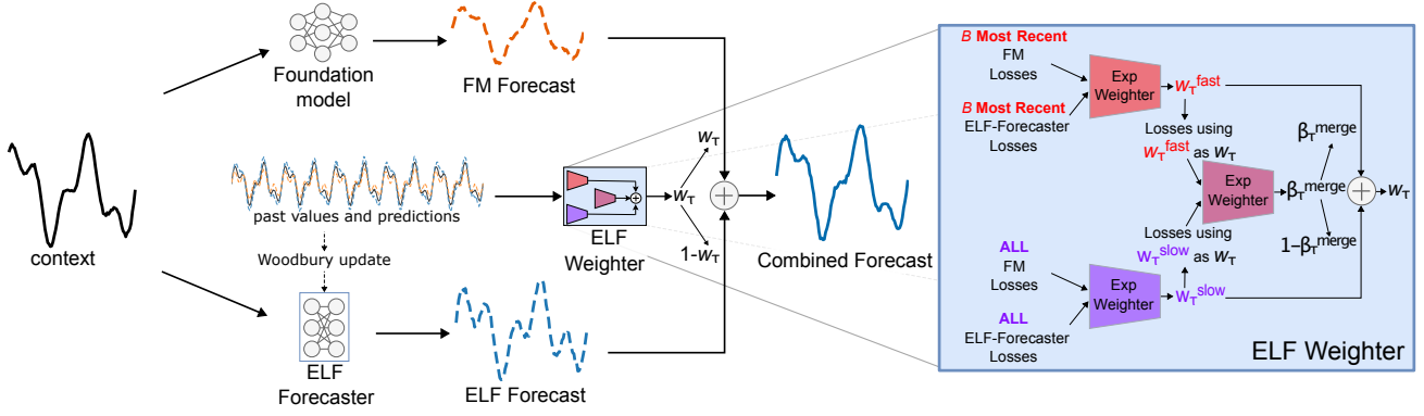
Figure 4. Forecast construction for FM+ELF: The left side of the figure shows how ELF adjusts the forecast of the FM. This is achieved by combining the FM forecast with the forecasts of the online (Woodbury) updated ELF-Forecaster using a weighted average. The weights w_T in the weighted average are determined by the ELF-Weighter based on previous performance of the FM and ELF-Forecaster. The schematic in the blue box to the right, zooms into the components of the ELF-Weighter: the fast, slow and merge weighters. Where the fast weighter gives a weighting based on recent performance; the slow weighter gives a weighting based on performance across the whole history. The merge weighter is used to combine the weights given by the fast and slow weighters. Each weighter uses exponential weighting to construct their weights; the difference being the losses used as input. While the slow weighter can be seen as using all previous losses to compute its weight, we note that only the last B losses need to be stored by ELF.
