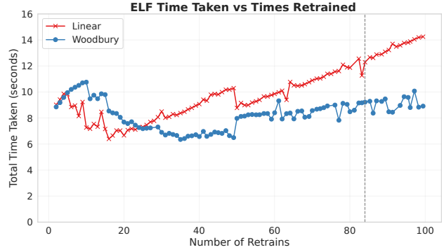
Figure 7. The impact of retraining frequency on ELF fitting+inference speed: We plot the total time taken for fitting and inference in ELF as we vary the number of times the model is refitted during evaluation on the ETTh1 dataset with a horizon of 336. We compare the performance of the Woodbury update rule (blue) with the more basic OLS (‘linear’) approach. No frequency components are removed in this experiment. As retraining becomes more frequent, the benefit of using the Woodbury identity increases; when retraining occurs 84 times, the speed-up is approximately 25% over the naive ‘linear’ implementation. Minor fluctuations in the curve reflect the noise inherent in measuring computation speed.
