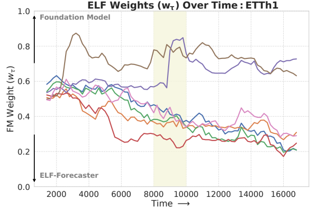
Figure 2. Each line in the plot show the ELF weight ( w_\tau ) over time for the Chronos FM for each channel of the ETTh1 dataset: A weight of 1 means that the ELF-Forecaster has no contribution to the final forecast, similarly, a weight of 0 means that the FM is not contributing to the final forecast. The plot shows that usually the FM weights gradually decrease; this reflects the fact that as the ELF-Forecaster observes more data its performance improves and it is upweighted by the ELF-Weighter. Occasionally, the weights adapt quickly to changes in the underlying time series, for example the purple channel shows a rapid weighting change between steps 8,000-10,000 (shaded in cream).
