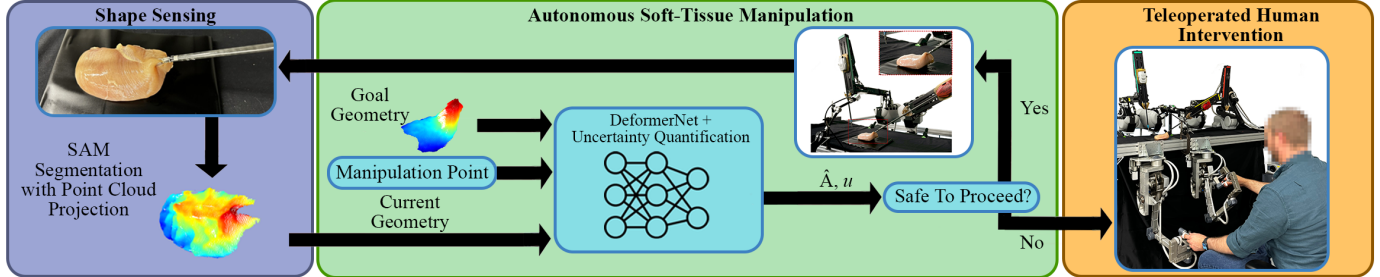
Fig. 1: Overall pipeline and experimental setup. We sense a point cloud of the current geometry of the tissue using the Segment Anything Model (SAM) [23] to segment RGBD images of the scene. SAM takes as input the RGB components of the image along with a query point on the desired segmented object. The resulting segmentation mask is then converted into a point cloud using the depth component of the image along with the camera’s intrinsic matrix to give the three-dimensional geometry of the tissue. The current geometry, coupled with the goal geometry and manipulation point, are passed as input to a deep ensemble of DeformerNet [50] models to predict a robot action \hat{A} (homogeneous transformation matrix) and an uncertainty estimate u . Using u , we determine if it is safe for the daVinci Research Kit (dVRK) robot to take action \hat{A} . If yes, the robot takes action \hat{A} , and the process repeats. Otherwise, the system requests a human to intervene and complete the task. We perform human interventions using the surgeon-side dVRK manipulators for teleoperation.
