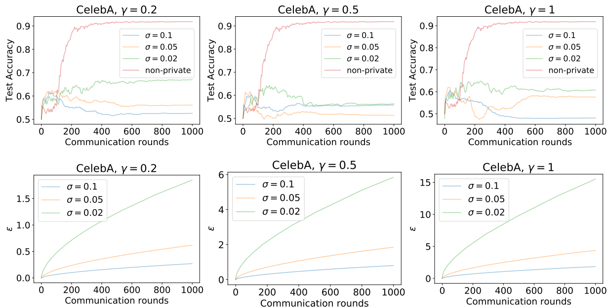
Figure 5: CelebA results
