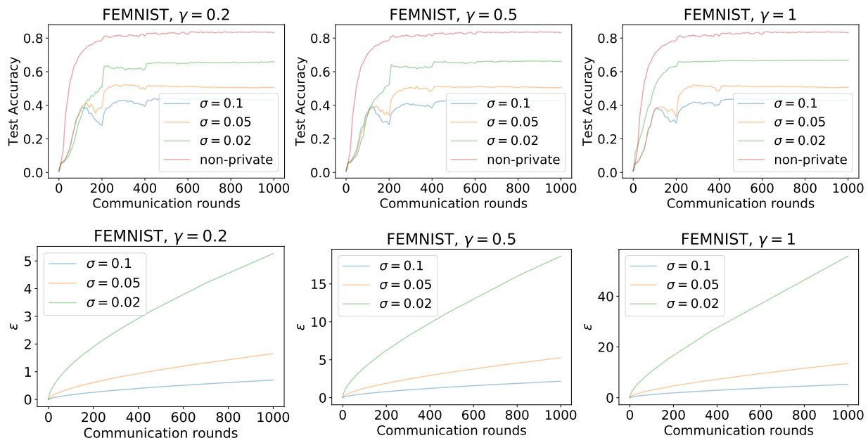
Figure 4: FEMNIST results
