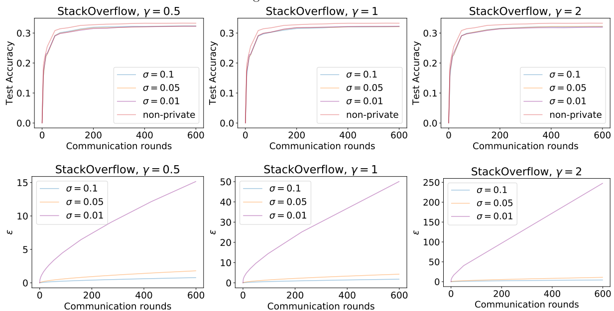
Figure 6: StackOverflow results
