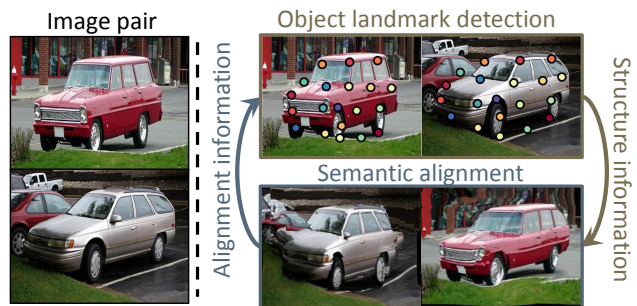
Figure 1. Illustration of the proposed joint learning framework: given only semantically similar image pairs, we address the crucial drawbacks of current weakly- or unsupervised models for the object landmark detection and semantic alignment task by alternatively leveraging mutual guidance information between them.
