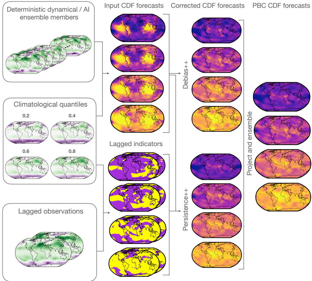
Figure 4: Probabilistic bias correction (PBC) schematic. PBC takes as input lagged observations, climatological quantiles, and the deterministic forecasts of any dynamical or AI model and outputs a learning-enhanced probabilistic forecast designed to correct systematic prediction errors.
