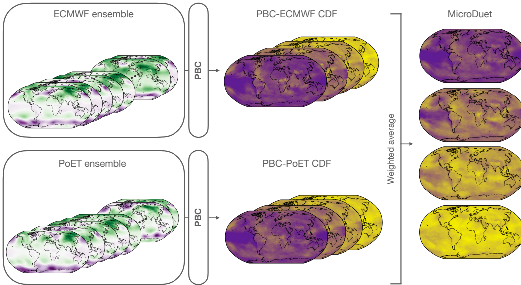
Figure 5: MicroDuet model schematic. MicroDuet outputs a weighted average of probabilistic bias correction (PBC) applied to the leading dynamical ensemble from ECMWF and the hybrid (AI + dynamical) PoET ensemble to leverage the complementary strengths of each.
