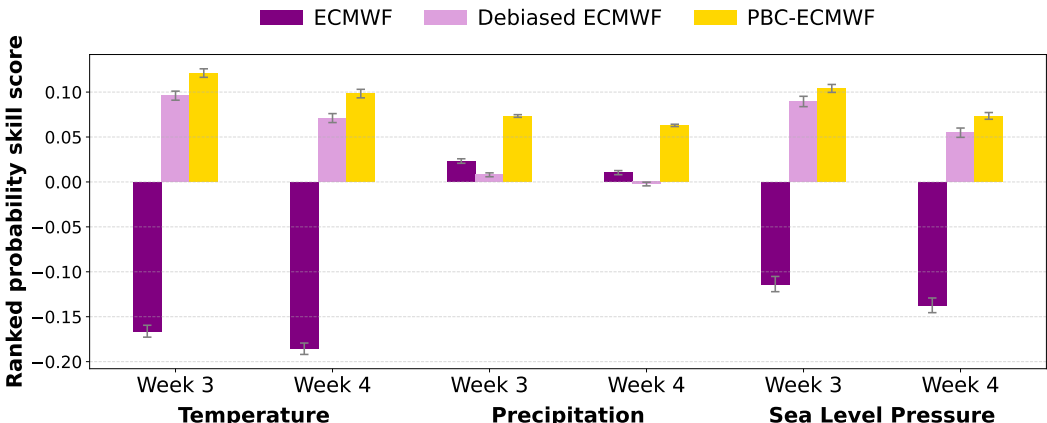
Figure 1: Average forecast skill of the leading dynamical model (ECMWF) and its probabilistic bias correction (PBC). Across the globe and the years 2016–2024, PBC boosts ECMWF skill more effectively than operational debiasing protocols for all variables and lead times.
