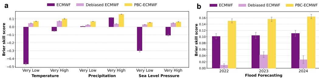
Figure 3: Forecasting extreme weather with the leading dynamical model (ECMWF) and its probabilistic bias correction (PBC) in week 4. (a) Across the globe and the years 2016–2024, PBC boosts ECMWF extreme weather forecasting skill more effectively than operational debiasing protocols for every variable and extreme. (b) Across flood events catalogued by the Global Disaster Awareness and Coordination System, operational debiasing severely degrades flood forecasting skill (top precipitation quintile Brier skill score in the 20^\circ \times 20^\circ bounding box centered on the flood), while PBC consistently enhances it.
