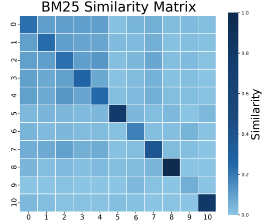
Figure 3: BM25 similarity matrix among retrieved documents, where D0-D4 are poisoned, and D5-D10 are clean.
