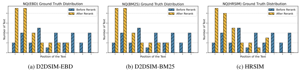
Figure 14: Distribution of Ground Truth document positions after applying GRADA in the NQ dataset with different ranking methods.
