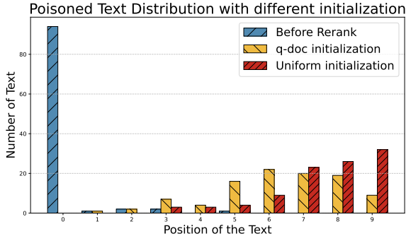
(a) Distribution of Poisoned document positions after applying GRADA (HRSIM) with different initialization in the NQ dataset.
